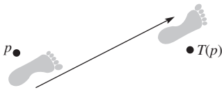
Figure 27.2 Glide-reflection
