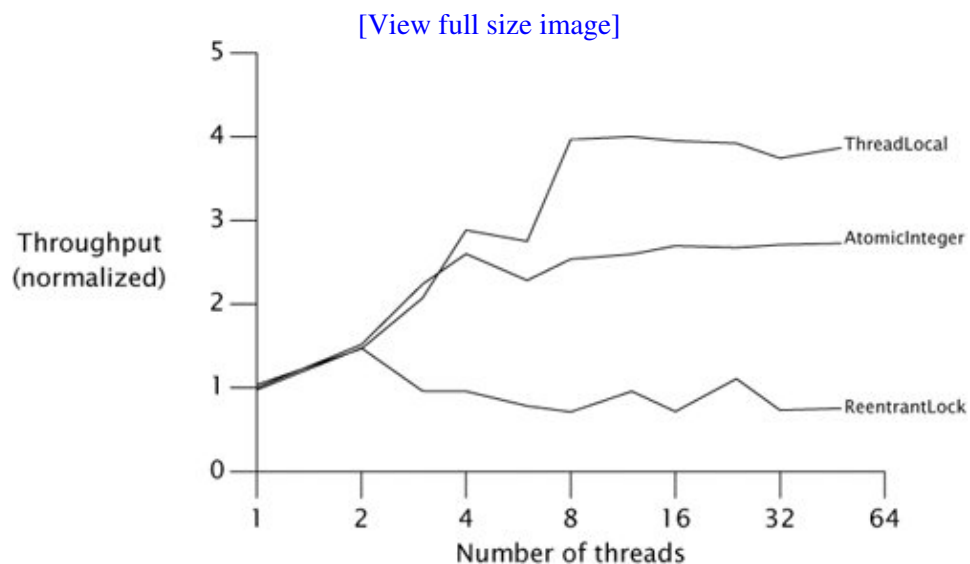
Figure 15.2. Lock and AtomicInteger Performance Under Moderate Contention.
