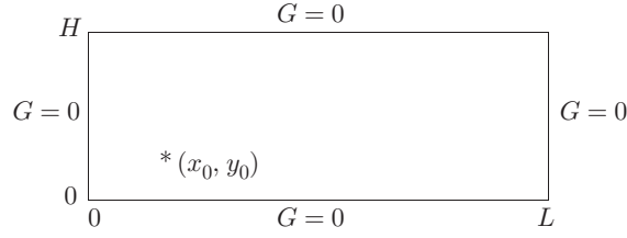
FIGURE 5.2 Green's function for Poisson's equation on a rectangle.
