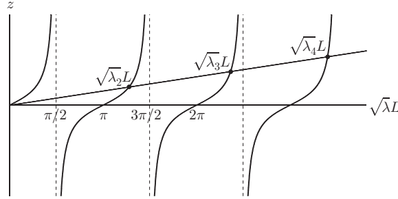
FIGURE 8.4 Positive eigenvalues ( hL < -1 ).
