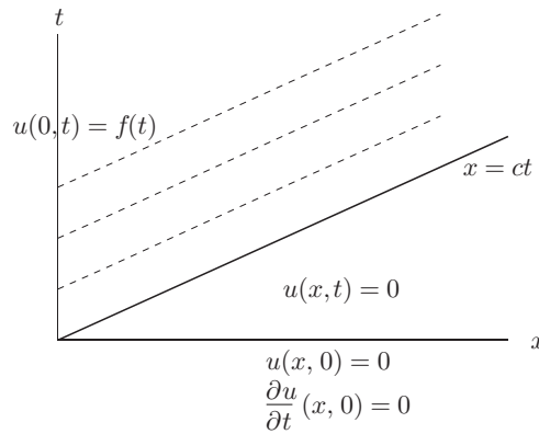
FIGURE 4.1 Signal problem for the one-dimensional wave equation.
