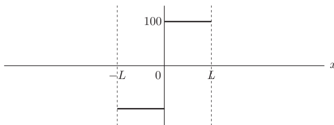
FIGURE 3.3 Odd extension of f(x) = 100 .
