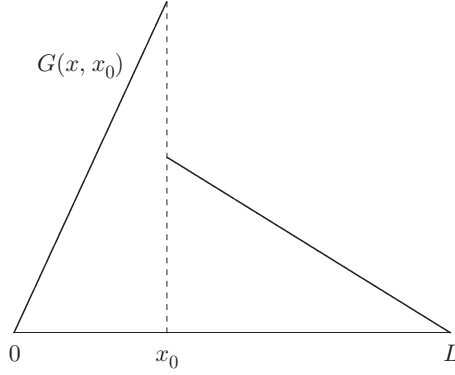
FIGURE 3.4 Green's function before application of jump conditions at x = x_0 .
