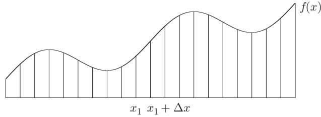
FIGURE 3.1 Piecewise constant representation of a typical function.
