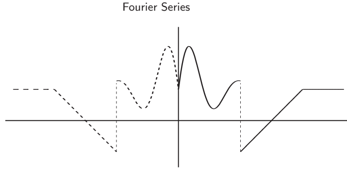
FIGURE 3.12 Even extension of f(x) .
