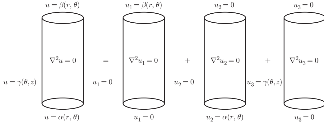
FIGURE 9.1 Laplace's equation in a circular cylinder.
