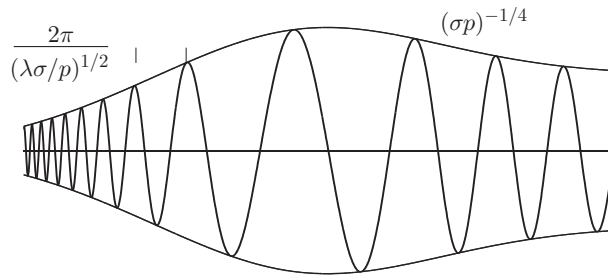
FIGURE 9.1 Liouville–Green asymptotic solution of differential equation showing rapid oscillation (or, equivalently, relatively slowly varying amplitude).
