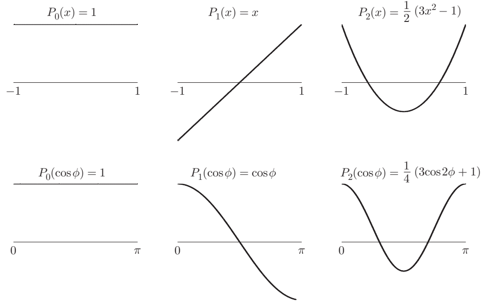
FIGURE 10.1 Legendre polynomials.
