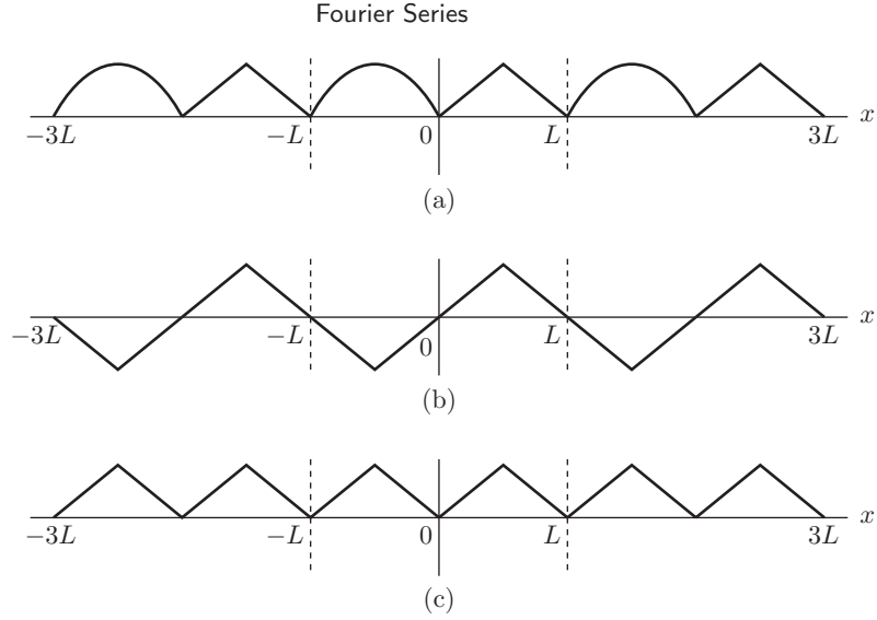
FIGURE 3.16 (a) Fourier series of f(x) ; (b) Fourier sine series of f(x) ; (c) Fourier cosine series of f(x) .
