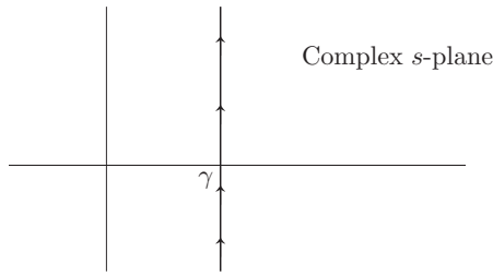
FIGURE 7.1 Line integral in complex s -plane for inverse Laplace transforms.
