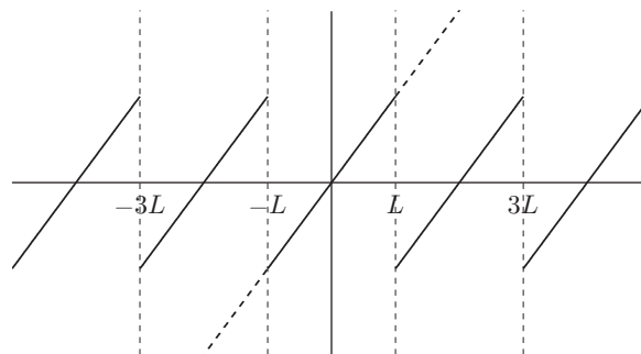
FIGURE 1.4 Periodic extension of f(x) = \frac{3}{2}x .
