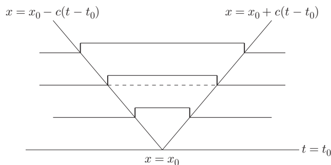
FIGURE 2.2 Green's function for the one-dimensional wave equation.
