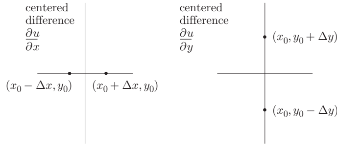
FIGURE 2.3 Points for first partial derivatives.
