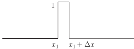
FIGURE 3.2 Pulse with unit height.
