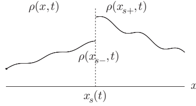
FIGURE 6.8 Density discontinuity at x = x_s(t) .
