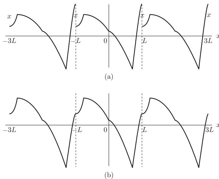
FIGURE 3.17 Fourier series of a continuous function with (a) f(-L) \neq f(L) and (b) f(-L) = f(L) .
