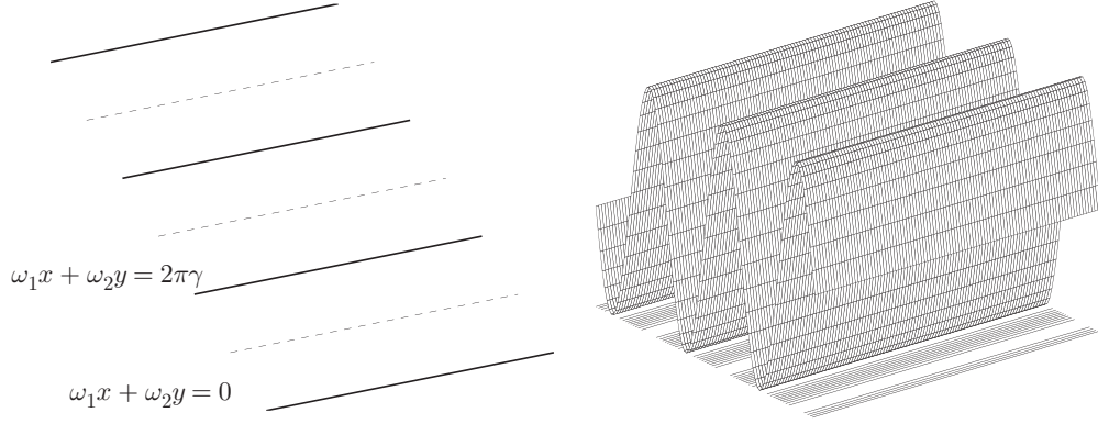
FIGURE 6.4 Two-dimensional wave and its crests.
