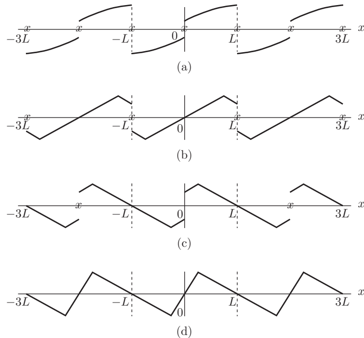
FIGURE 3.19 Fourier sine series of a continuous function with (a) f(0) \neq 0 and f(L) \neq 0 ; (b) f(0) = 0 but f(L) \neq 0 ; (c) f(L) = 0 but f(0) \neq 0 ; and (d) f(0) = 0 and f(L) = 0 .
