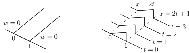
FIGURE 2.2 Propagation for the first-order wave equation.
