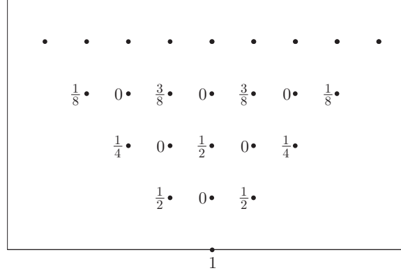
FIGURE 3.7 Pascal's triangle.
