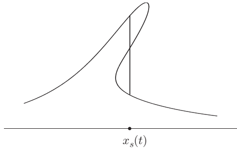
FIGURE 6.15 Whitham's equal-area principle.
