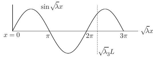
FIGURE 8.5 Zeros of the eigenfunctions \sin \sqrt{\lambda}x .
