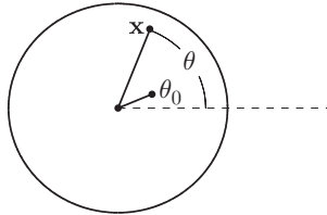
FIGURE 5.5 Polar coordinates.
