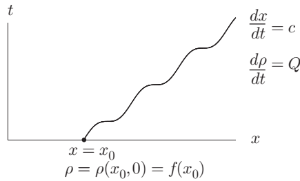
FIGURE 6.1 Characteristic starting from x = x_0 at time t = 0 .
