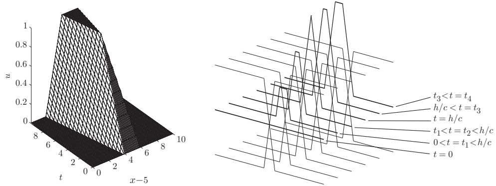
FIGURE 3.4 Time evolution for a struck string.
