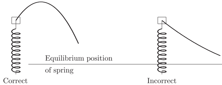
FIGURE 3.2 Boundary conditions for massless spring-mass system.
