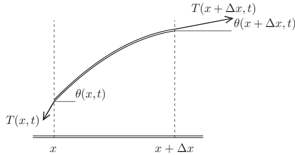
FIGURE 2.2 Stretching of a finite segment of string, illustrating the tensile forces.
