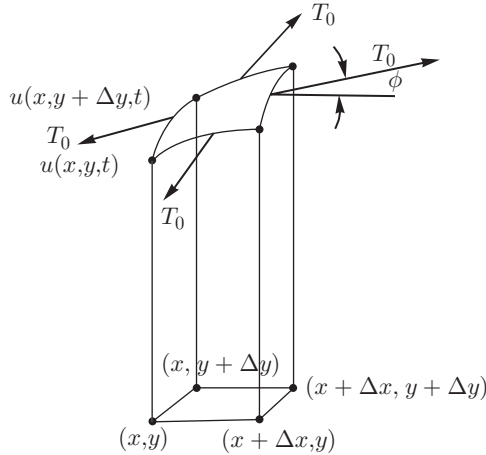
FIGURE 5.1 Slightly stretched membrane with approximately constant tension T_0 .
