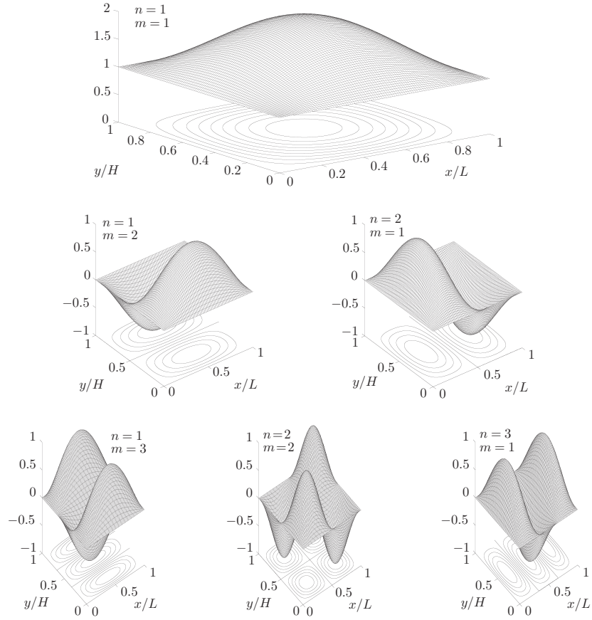
FIGURE 3.2 Nodal curves for modes of a vibrating rectangular membrane.
