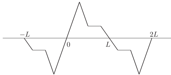
FIGURE 5.3 Odd-periodic extension.
