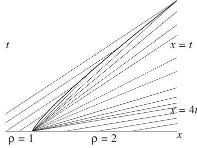
FIGURE 6.11 Characteristics for shock and expansion wave.
