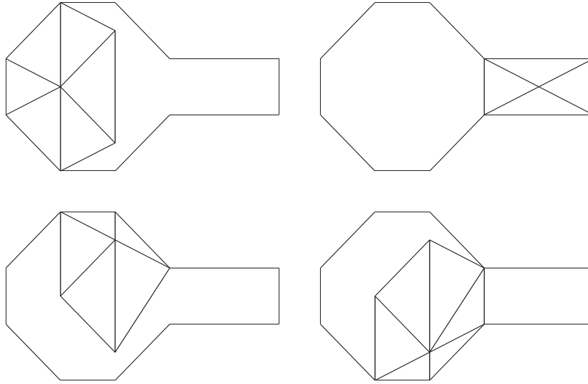
FIGURE 7.3 Four trial functions (one corresponds to each interior point).
