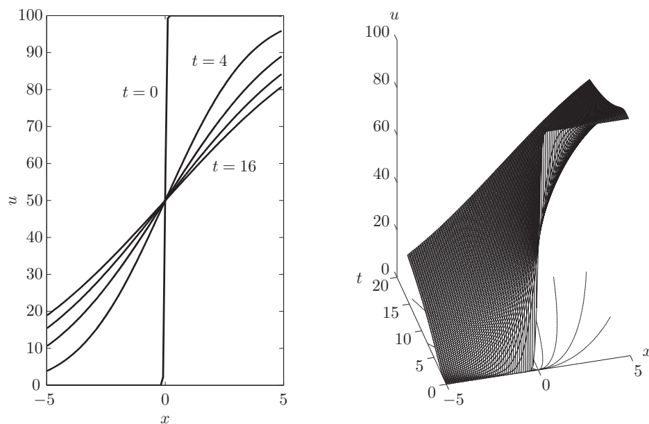
FIGURE 4.4 Temperature diffusion in an infinite rod.
