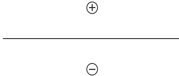
FIGURE 5.3 Image source for a semi-infinite plane.
