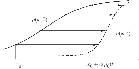
FIGURE 6.3 Graphical solution.
