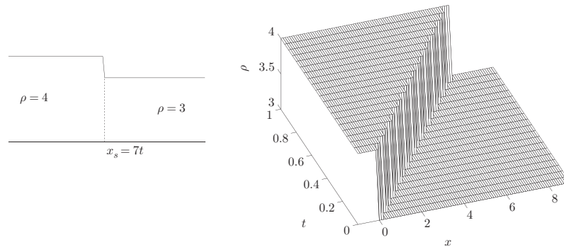
FIGURE 6.10 Density shock wave.
