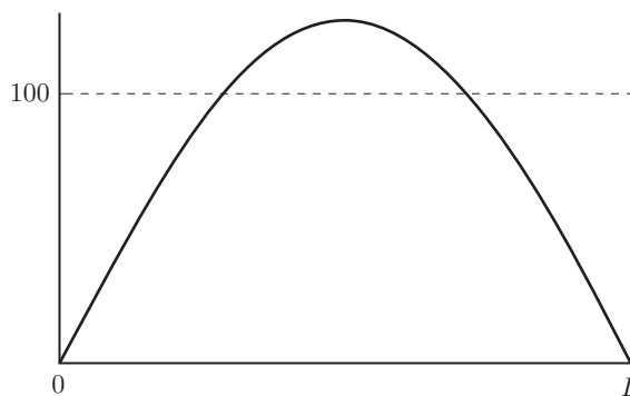
FIGURE 3.6 First term of Fourier sine series of f(x) = 100 .
