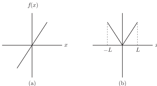
FIGURE 3.13 (a) f(x) = x , (b) its even extension.
