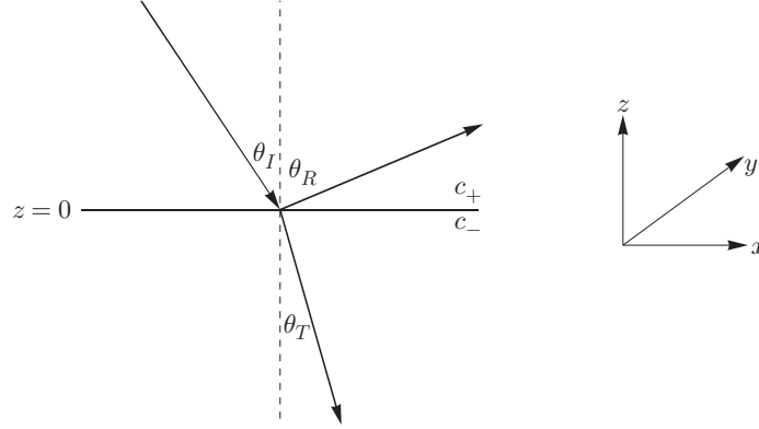
FIGURE 6.1 Reflected and refracted (transmitted) waves.
