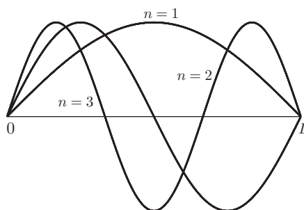
FIGURE 3.3 Eigenfunctions \sin n\pi x/L and their zeros.
