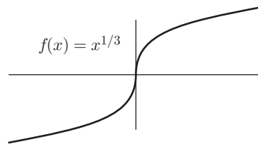
FIGURE 1.3 Example of a function that is not piecewise smooth.
