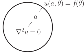
FIGURE 5.2 Laplace's equation inside a circular disk.
