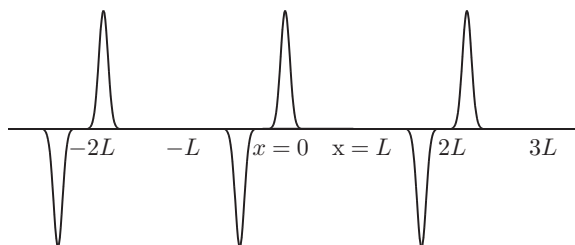
FIGURE 3.1 Multiple image sources for the Green's function for the heat equation for a finite one-dimensional rod.
