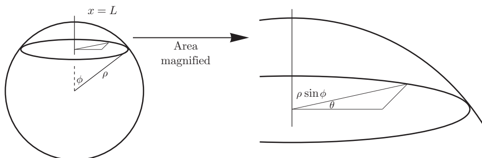
FIGURE 5.3 Spherical coordinates.
