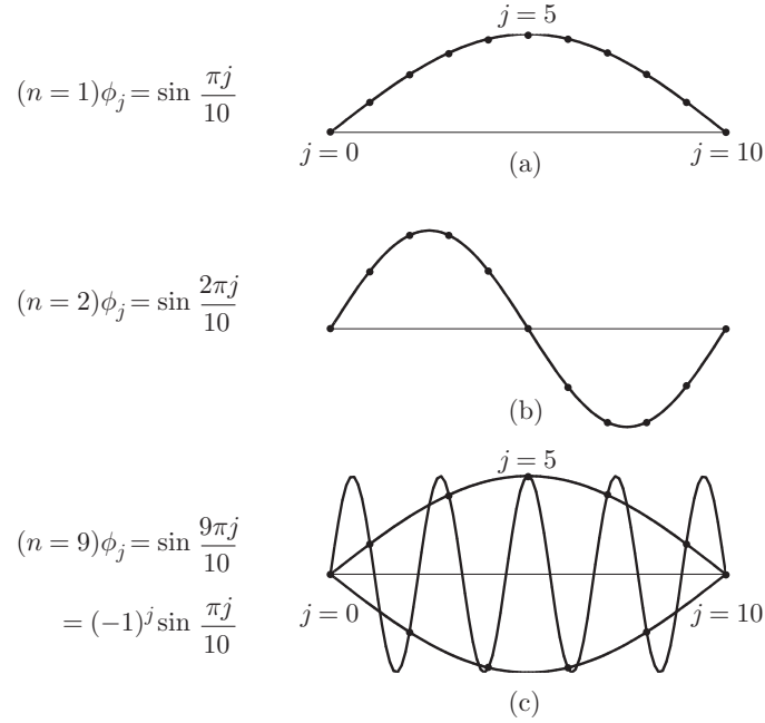
FIGURE 3.6 Eigenfunctions for the discrete problem.
