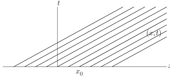
FIGURE 2.1 Characteristics for the first-order wave equation.
