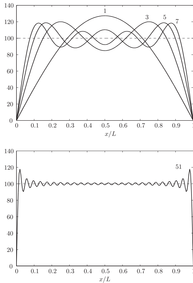
FIGURE 3.8 Various partial sums of Fourier sine series of f(x) = 100 . Using 51 terms (including n = 51 ), the finite series is a good approximation to f(x) = 100 away from the endpoints. Near the endpoints (where there is a jump discontinuity of 200, there is a 9% overshoot (Gibbs phenomenon).
