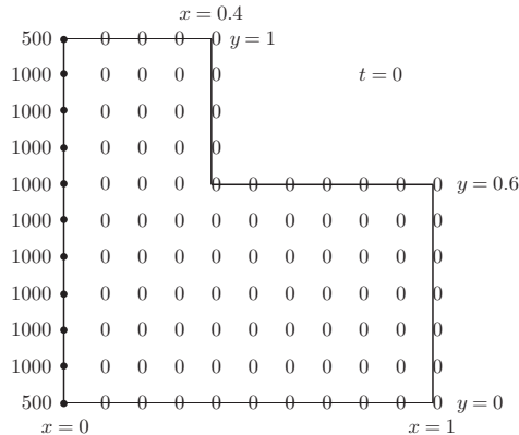
FIGURE 4.1 Initial condition.
