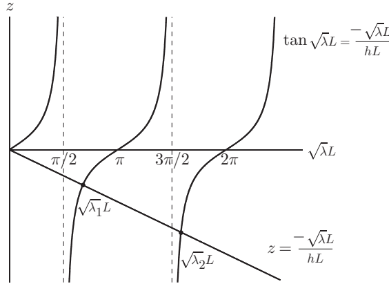
FIGURE 8.1 Graphical determination of positive eigenvalues ( h > 0 ).
