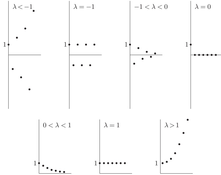
FIGURE 3.8 Solutions of first-order difference equations.
