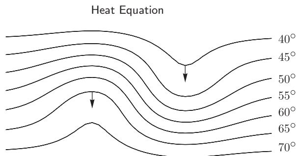
FIGURE 5.4 The gradient is perpendicular to level surfaces of the temperature.
