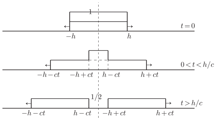
FIGURE 3.2 Initial value problem for the one-dimensional wave equation.
