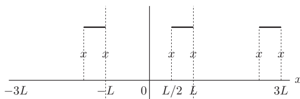
FIGURE 2.2 Fourier series of f(x) .
