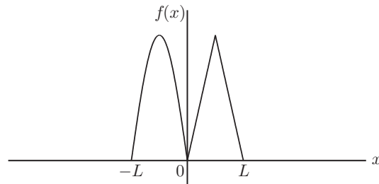
FIGURE 3.15 The graph of f(x) for -L < x < L .
