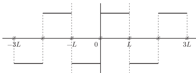
FIGURE 3.4 Fourier sine series of f(x) = 100 .
