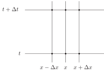
FIGURE 3.10 Implicit Crank–Nicolson scheme.
