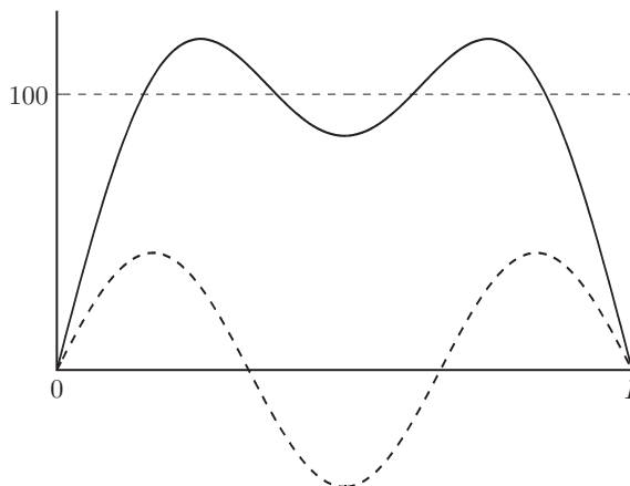
FIGURE 3.7 First two nonzero terms of Fourier sine series of f(x) = 100 .
