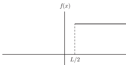
FIGURE 2.1 Sketch of f(x) .
