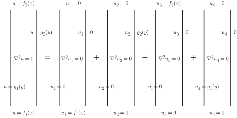
FIGURE 5.1 Laplace's equation inside a rectangle.
