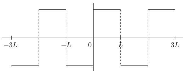
FIGURE 4.3 Fourier sine series of df/dx .
