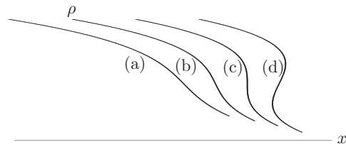
FIGURE 6.7 Density wave steepens (density becomes triple valued).
