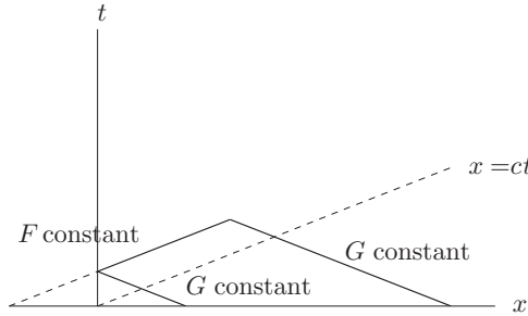
FIGURE 4.3 Reflected characteristics.
