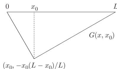
FIGURE 3.5 Green's function.
