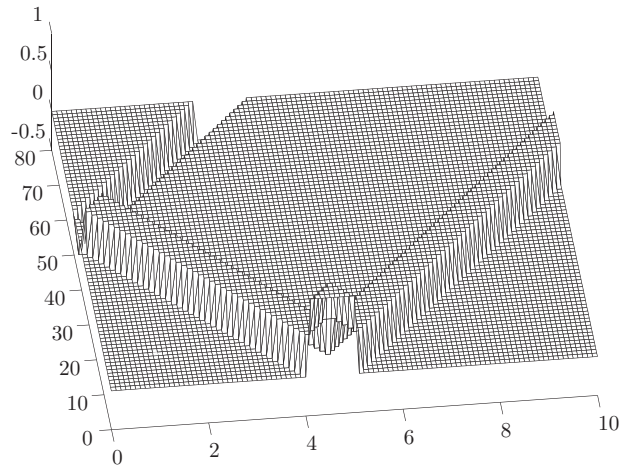
FIGURE 4.4 Reflected pulse.
