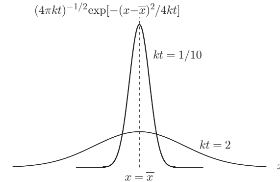
FIGURE 4.1 Fundamental solution for the heat equation.
