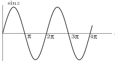
FIGURE 3.1 Zeros of \sin z .
