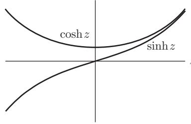
FIGURE 3.2 Hyperbolic functions.
