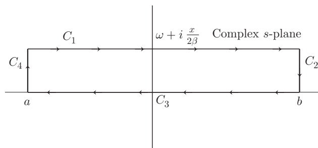
FIGURE 3.3 Closed contour integral in the complex plane.
