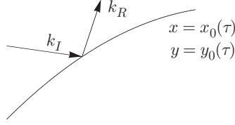
FIGURE 7.1 Reflected wave from curved boundary.
