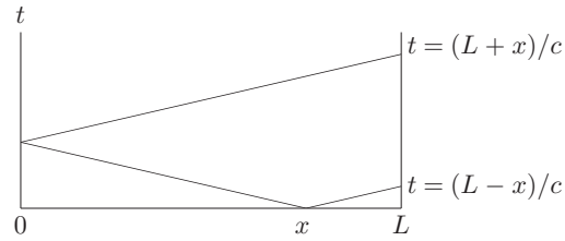
FIGURE 5.1 Space-time signal paths.
