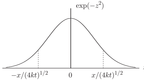
FIGURE 4.2 Area under a Gaussian.
