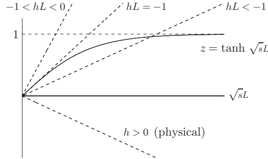
FIGURE 8.3 Graphical determination of negative eigenvalues.
