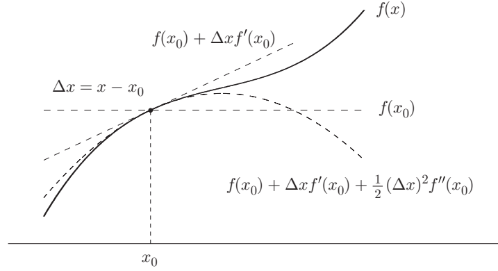
FIGURE 2.1 Taylor polynomials.
