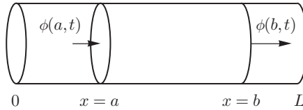
FIGURE 2.2 Heat energy flowing into and out of a finite segment of a rod.
