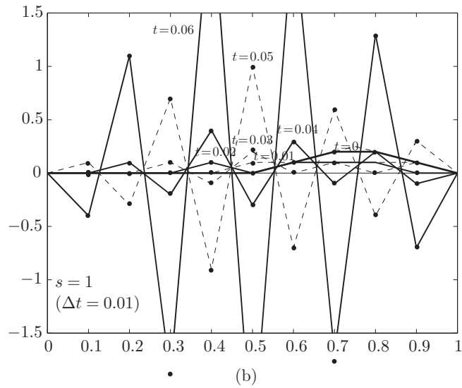
FIGURE 3.5 Computations for the heat equation s = k(\Delta t)/(\Delta x)^2 : (a) s = \frac{1}{4} stable and (b) s = 1 unstable.
