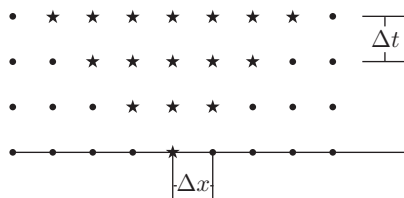
FIGURE 3.3 Propagation speed of disturbances.
