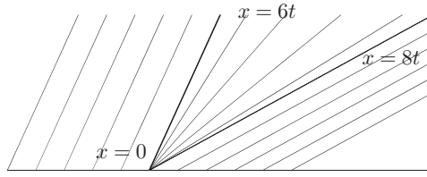
FIGURE 6.4 Characteristics (including the fanlike ones).
