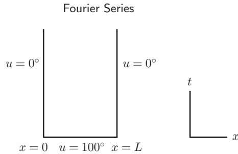
FIGURE 3.5 Boundary and initial conditions.
