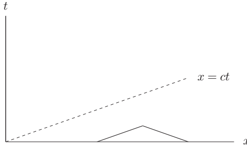
FIGURE 4.2 Characteristics.
