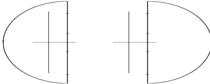
FIGURE 7.2 Closing the line integrals.
