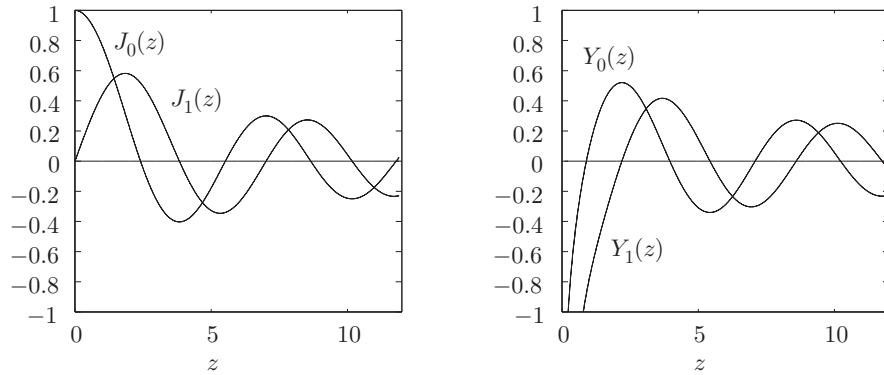
FIGURE 8.1 Sketch of various Bessel functions.
