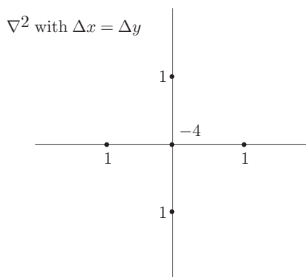
FIGURE 2.4 Weights for the Laplacian ( \Delta x = \Delta y ).
