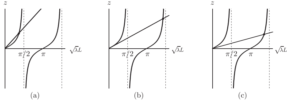
FIGURE 8.2 Graphical determination of positive eigenvalues: (a) 0 > hL > -1 ; (b) hL = -1 ; (c) hL < -1 .
