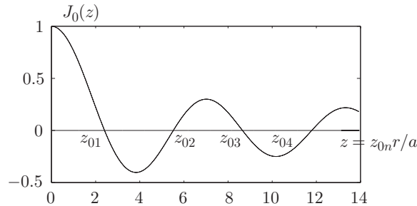
FIGURE 8.2 Sketch of J_0(z) and its zeros.
