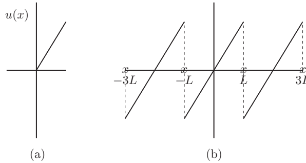
FIGURE 3.9 (a) f(x) = x and (b) its Fourier sine series.
