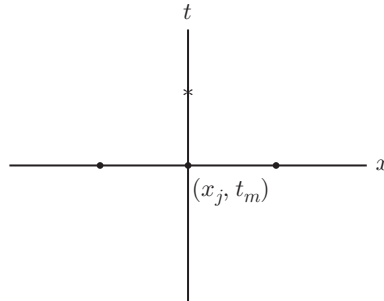
FIGURE 3.2 Marching forward in time.
