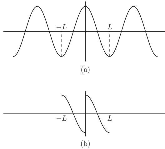
FIGURE 3.10 (a) f(x) = \cos \pi x/L and (b) its odd extension.
