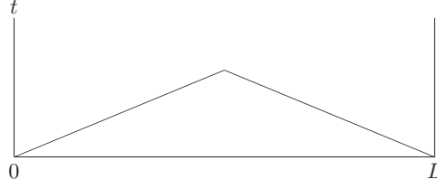
FIGURE 5.1 Characteristics.
