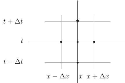
FIGURE 5.1 Marching forward in time for the wave equation.
