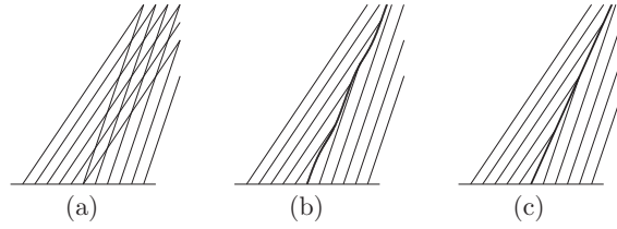
FIGURE 6.9 Shock caused by intersecting characteristics.
