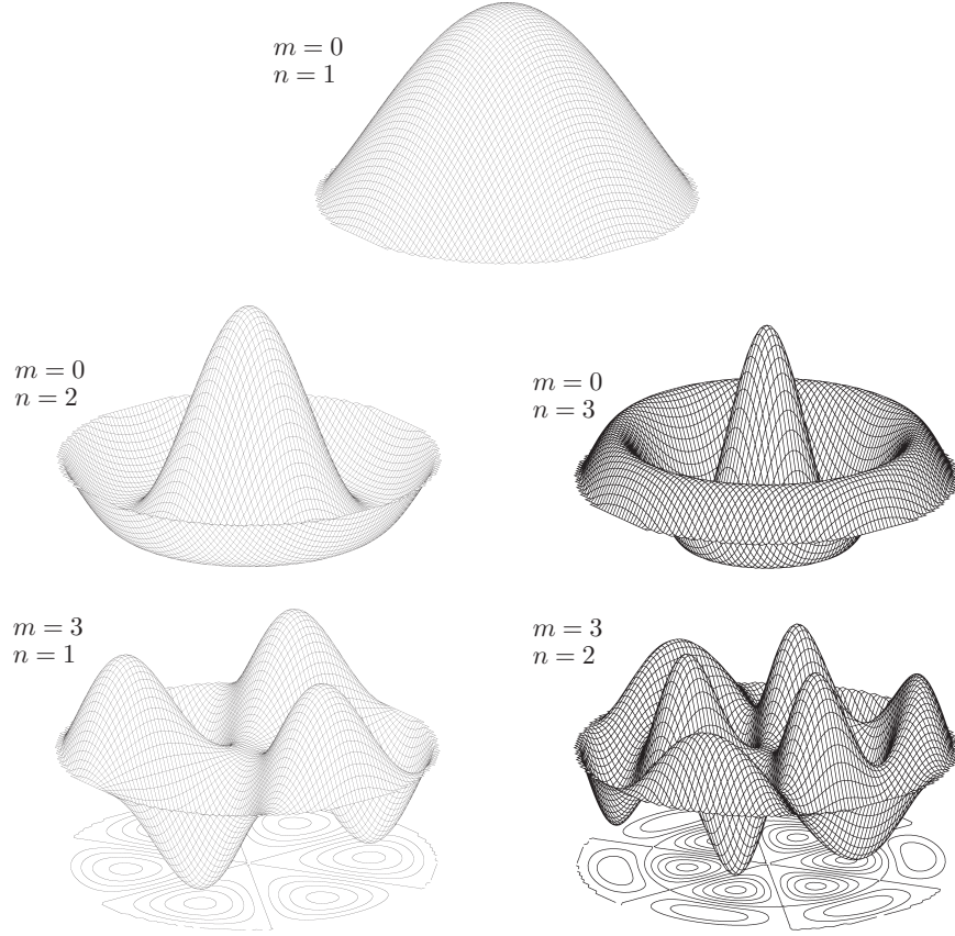
FIGURE 8.3 Normal nodes and nodal curves for a vibrating circular membrane.
