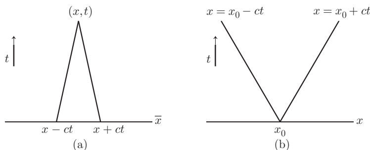
FIGURE 3.5 (a) Domain of dependence; (b) range of influence.
