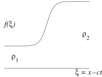
FIGURE 6.13 Spatial structure for traveling shock wave.
