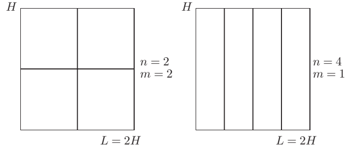
FIGURE 4.1 Nodal curves for eigenfunctions with the same eigenvalue (symmetric).
