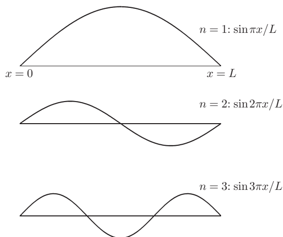
FIGURE 3.1 Zeros of eigenfunctions \sin n\pi x/L .
