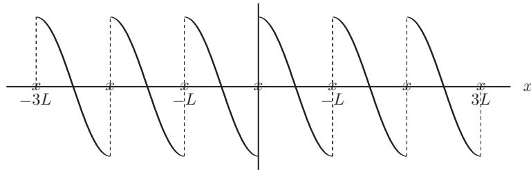
FIGURE 3.11 Fourier sine series of f(x) = \cos \pi x/L .
