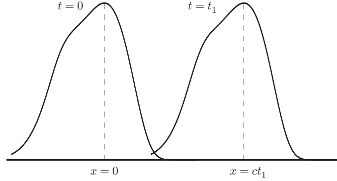
FIGURE 2.3 Shape invariance for the first-order wave equation.
