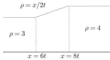
FIGURE 6.4 Characteristics (including the fanlike ones).
