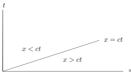
FIGURE 4.1 Characteristic emanating from the boundary.
