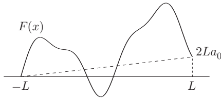
FIGURE 5.1 F(x) with F(-L) \neq F(L) .
