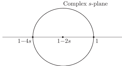
FIGURE 3.9 Gershgorin circles for \mathbf{A} corresponding to discretization of the heat equation.
