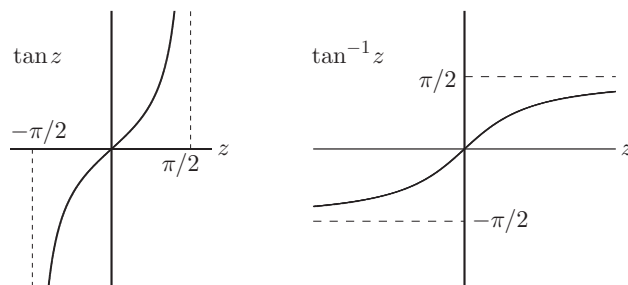
FIGURE 6.2 Tangent and inverse tangent functions.
