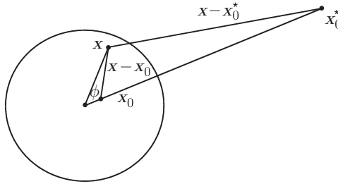
FIGURE 5.4 Green's function for Poisson's equation for a circle (image source).
