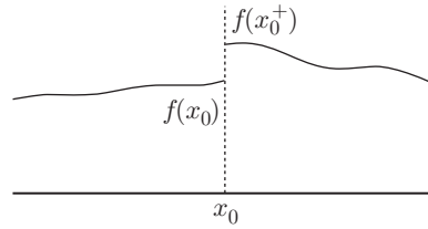
FIGURE 1.1 Jump discontinuity at x = x_0 .
