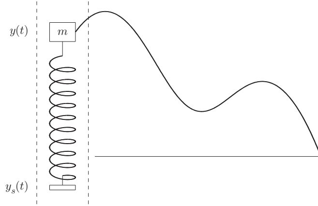
FIGURE 3.1 Spring-mass system with a variable support attached to a stretched string.
