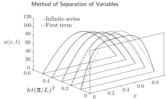
FIGURE 3.5 Time dependence of temperature (using the infinite series) compared to the first term. Note the first term is a good approximation if the time is not too small.
