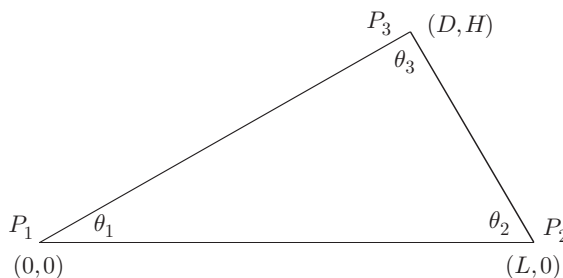
FIGURE 7.5 Triangular finite element.
