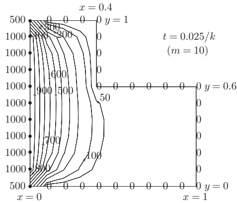
FIGURE 4.2 Numerical computation of temperature in an L -shaped region.
