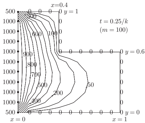
FIGURE 4.3 Numerical computation of temperature in an L -shaped region.
