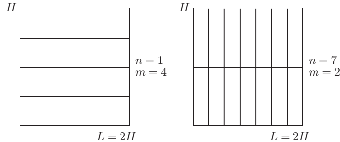
FIGURE 4.2 Nodal curves for eigenfunction with the same eigenvalue (asymmetric).
