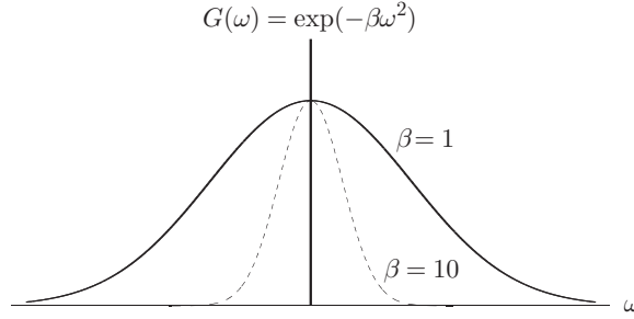
FIGURE 3.2 Bell-shaped Gaussian.
