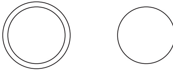
FIGURE 2.1 (a) Circular annulus; (b) circle.
