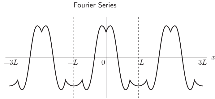
FIGURE 3.18 Fourier cosine series of a continuous function.
