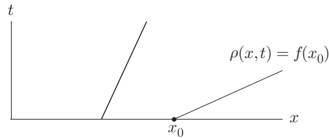
FIGURE 6.2 Possibly nonparallel straight-line characteristics.
