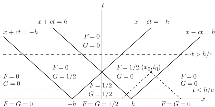
FIGURE 3.3 Method of characteristics for the one-dimensional wave equation.
