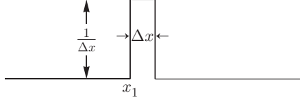
FIGURE 3.3 Rectangular pulse with unit area.
