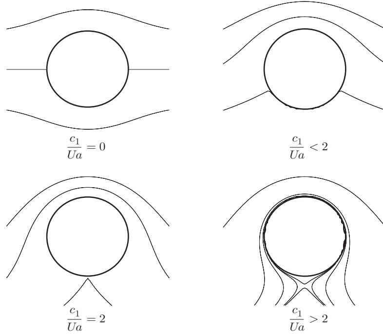
FIGURE 5.3 Flow past cylinder and lift = 2\pi\rho c_1 U .
