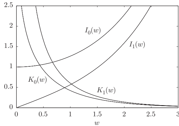
FIGURE 9.2 Various modified Bessel functions (from Abramowitz and Stegun, 1974).
