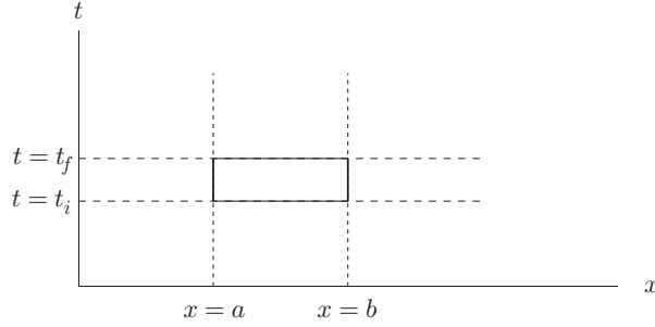
FIGURE 2.1 Space-time boundaries for a one-dimensional wave equation.
