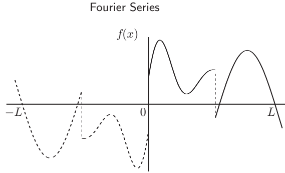
FIGURE 3.2 Odd extension of f(x) .
