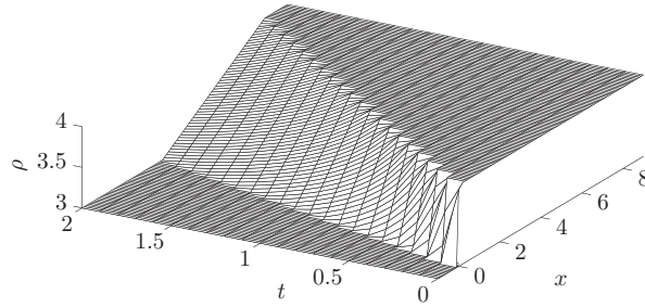
FIGURE 6.5 Expansion wave.
