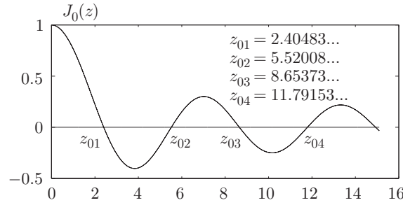
FIGURE 7.1 Sketch of J_0(z) and its zeros.
