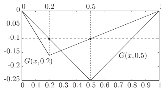
FIGURE 3.6 Illustration of Maxwell's reciprocity.
