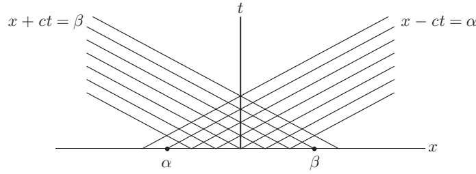
FIGURE 3.1 Characteristics for the one-dimensional wave equation.
