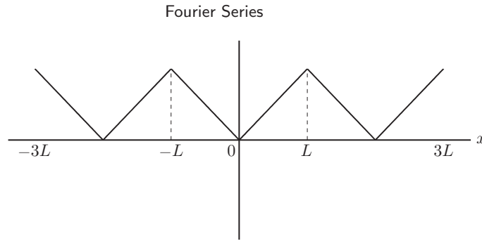
FIGURE 3.14 Fourier cosine series of the even extension of f(x) .
