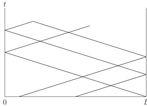
FIGURE 5.2 Multiply reflected characteristics.
