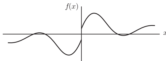
FIGURE 3.1 An odd function.
