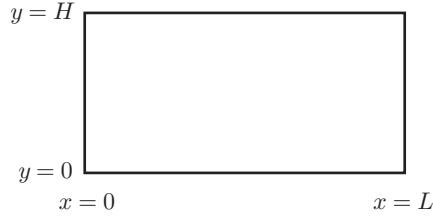
FIGURE 3.1 Rectangular membrane.
